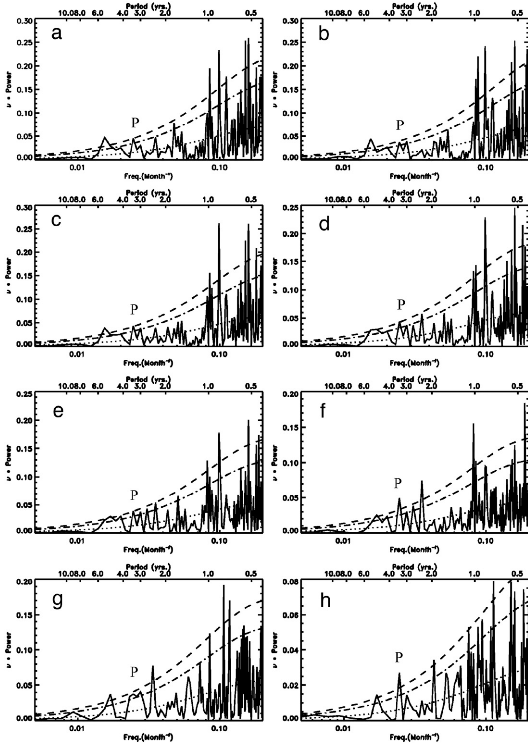
FIG. 6. Power spectra of the deseasonalized and detrended GEOS CCM \Omega_s data sampled at the same locations as those in Fig. 5. Dotted lines are the mean red noise spectra. Dashed-dotted lines and dashed lines are 10% and 5% significance levels, respectively; P denotes the 3.5-yr signal.
