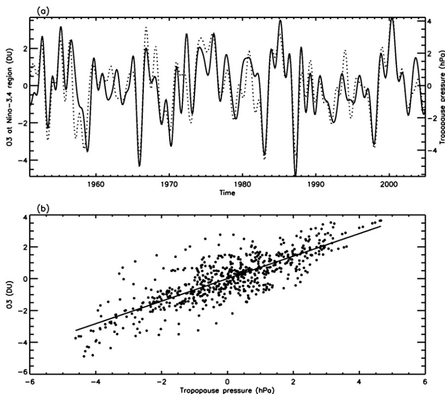
FIG. 4. (a) First mode of GEOS CCM \Omega_S averaged over the Niño-3.4 region (solid line) and first mode of GEOS CCM P_T averaged at the Niño-3.4 region (dotted line). Correlation coefficient between the two time series is 0.82 (0.1% significance level). (b) Scatterplot for GEOS CCM \Omega_S and P_T . Both data are averaged over the Niño-3.4 region. The solid line is the linear fit of the data.
