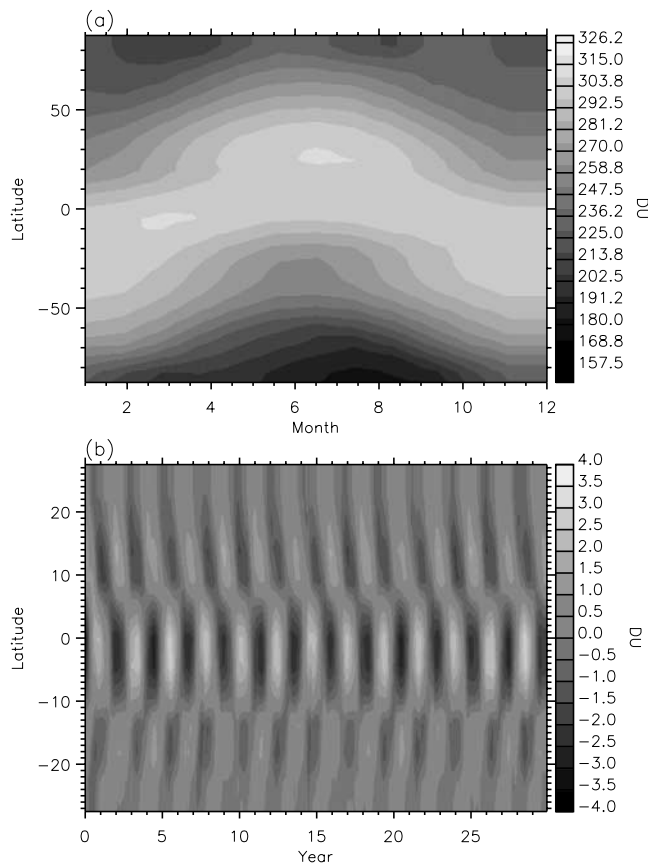
Figure 12. (a) Climatology and (b) anomaly of the total column ozone for experiment C. See color version of this figure at back of this issue.
