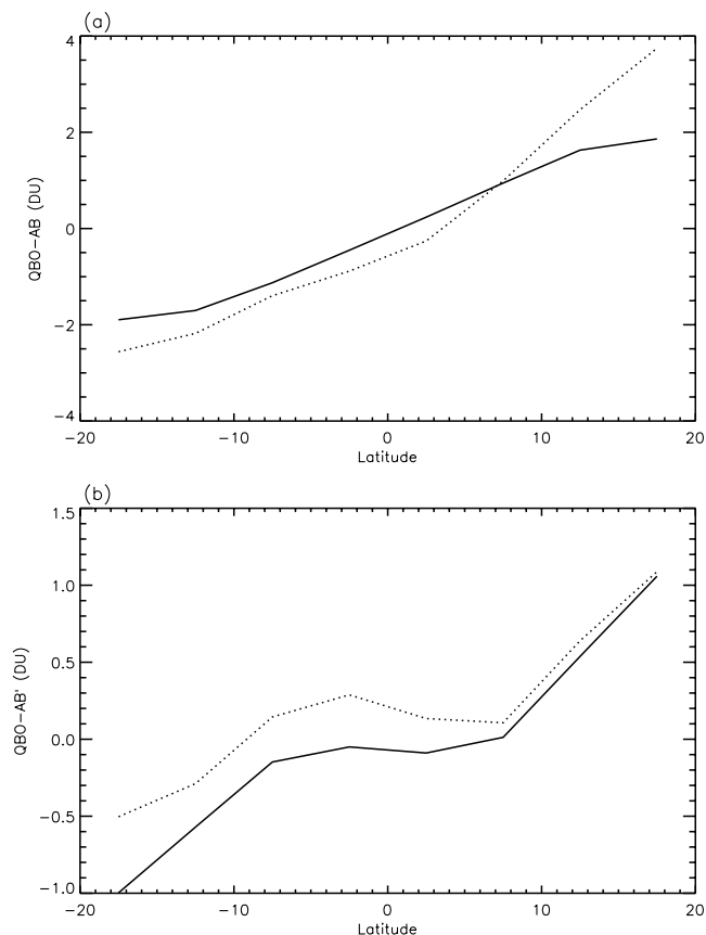
Figure 2. (a) Ozone QBO-AB and (b) QBO-AB' signals from 2-D chemistry and transport model (CTM) (solid line) and merged ozone data (MOD) (dotted line).
