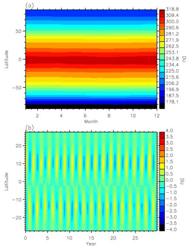
Figure 8. (a) Climatology and (b) anomaly of the total column ozone for experiment A.
