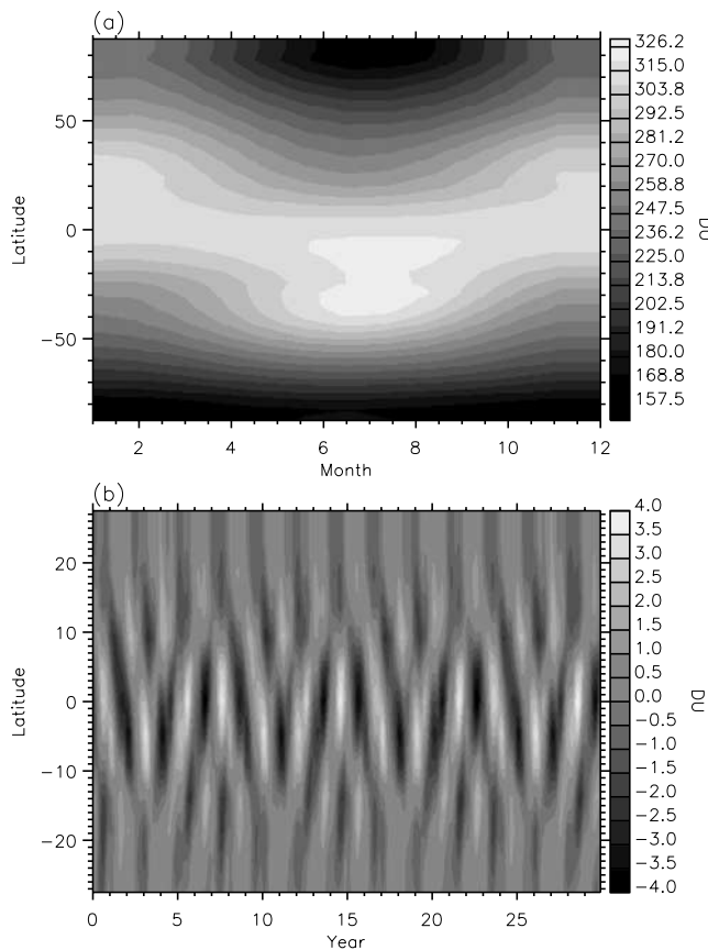
Figure 10. (a) Climatology and (b) anomaly of the total column ozone for experiment B. See color version of this figure at back of this issue.
