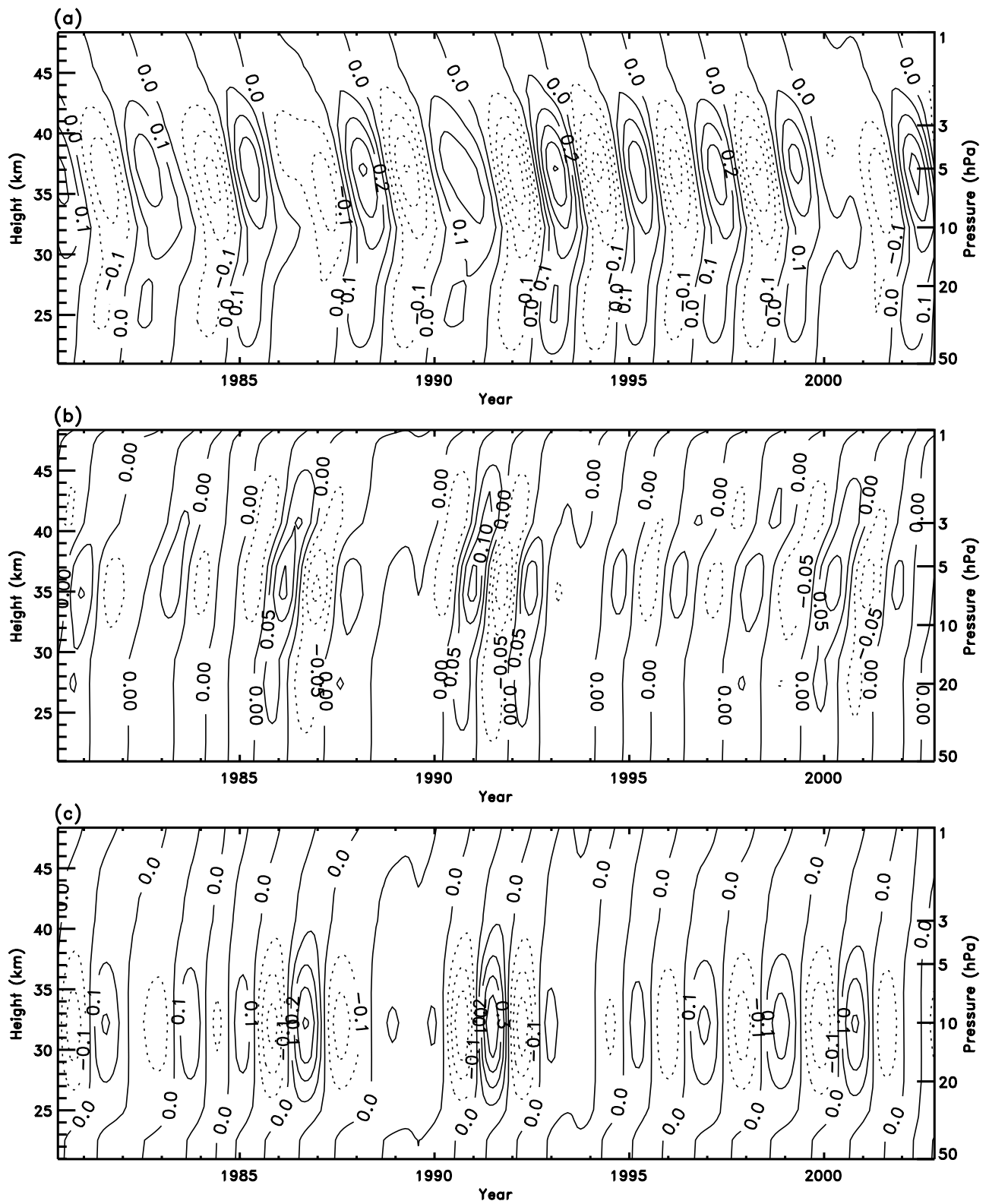
Figure 7. (a) PC_1 \times EEOF_1 + PC_2 \times EEOF_2 at equator, (b) PC_3 \times EEOF_3 + PC_4 \times EEOF_4 at 12.5^\circ\text{N} , and (c) PC_3 \times EEOF_3 + PC_4 \times EEOF_4 at 12.5^\circ\text{S} obtained at lag = 0 from the band-pass-filtered ozone VMR from MOD. Units are ppmv.
