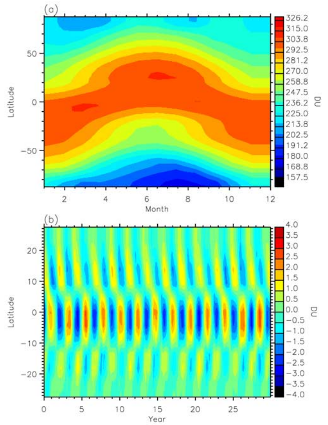
Figure 12. (a) Climatology and (b) anomaly of the total column ozone for experiment C.
