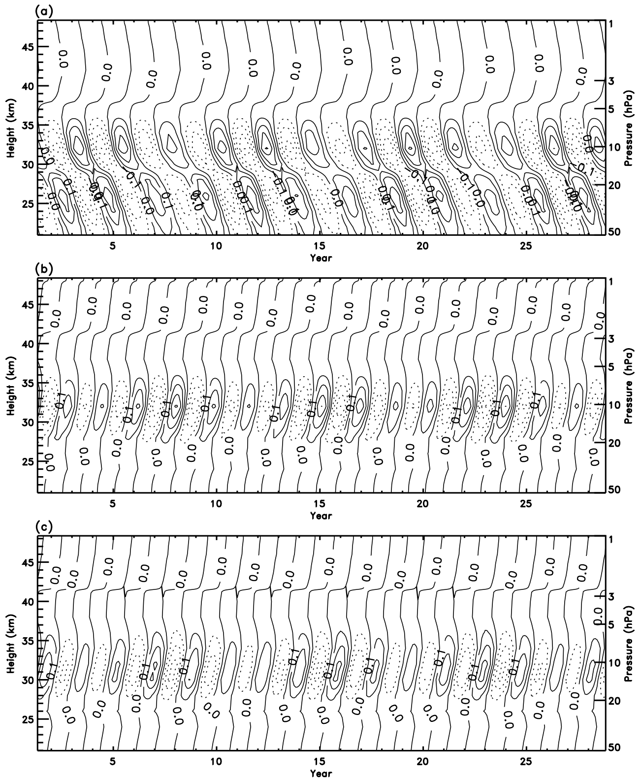
Figure 5. (a) PC_1 \times EEOF_1 + PC_2 \times EEOF_2 at equator, (b) PC_3 \times EEOF_3 + PC_4 \times EEOF_4 at 12.5^\circ N , and (c) PC_3 \times EEOF_3 + PC_4 \times EEOF_4 at 12.5^\circ S obtained at lag = 0 from the ozone VMR from the standard model. Units are ppmv.
